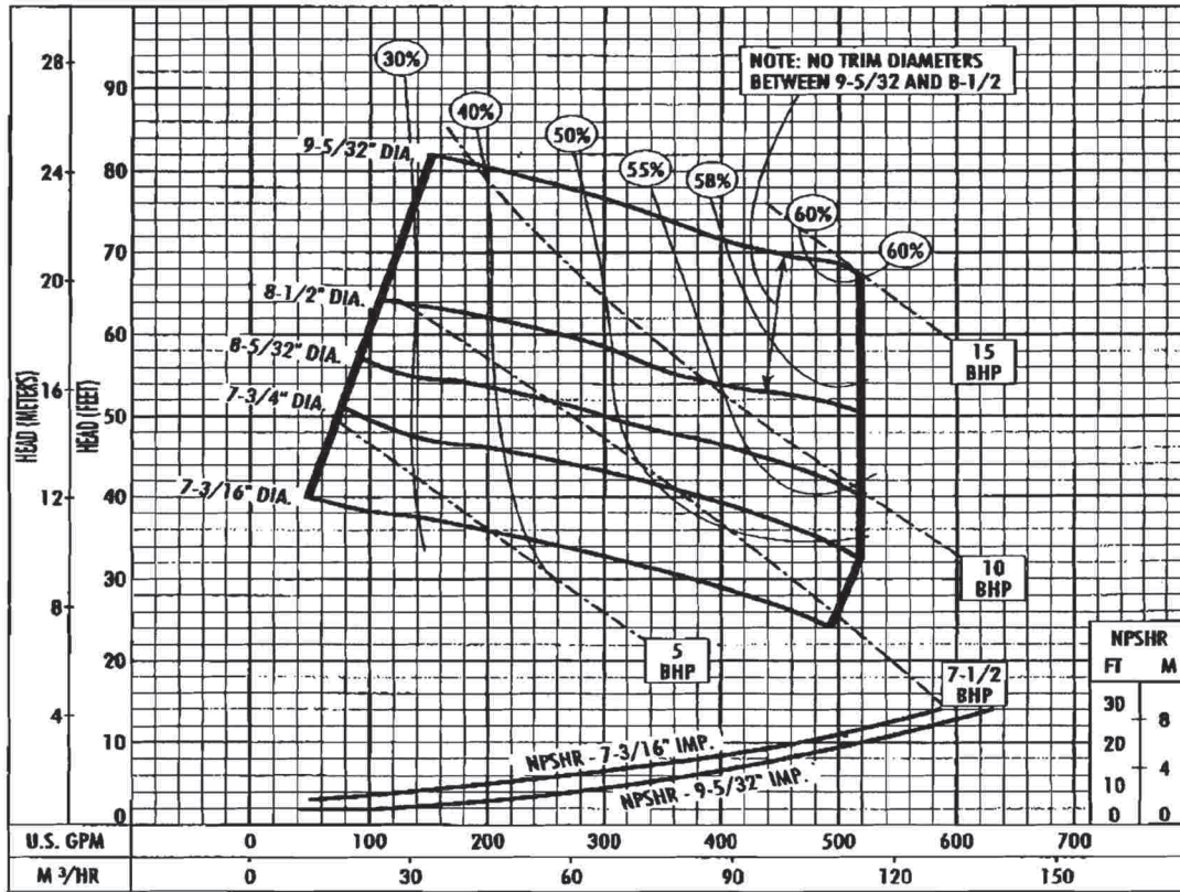
MT-4 PERFORMANCE CURVE @ 1750 RPM
